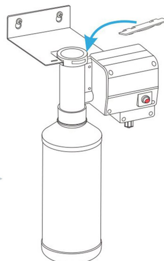
Insert the locking plate into bracket
